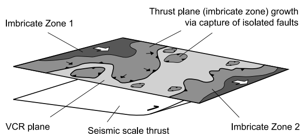
Fig. 17. Cartoon of the front of a propagating thrust imbricate zone (cf. Fig. 9). Isolated patches of faulting occur in advance of the tip line to the main imbrication, which grows by coalescing these isolated slip patches. Frontal and lateral ramps and footwall plucking structures develop to facilitate capture of slip patches ahead and above or below the main tip line, respectively.
